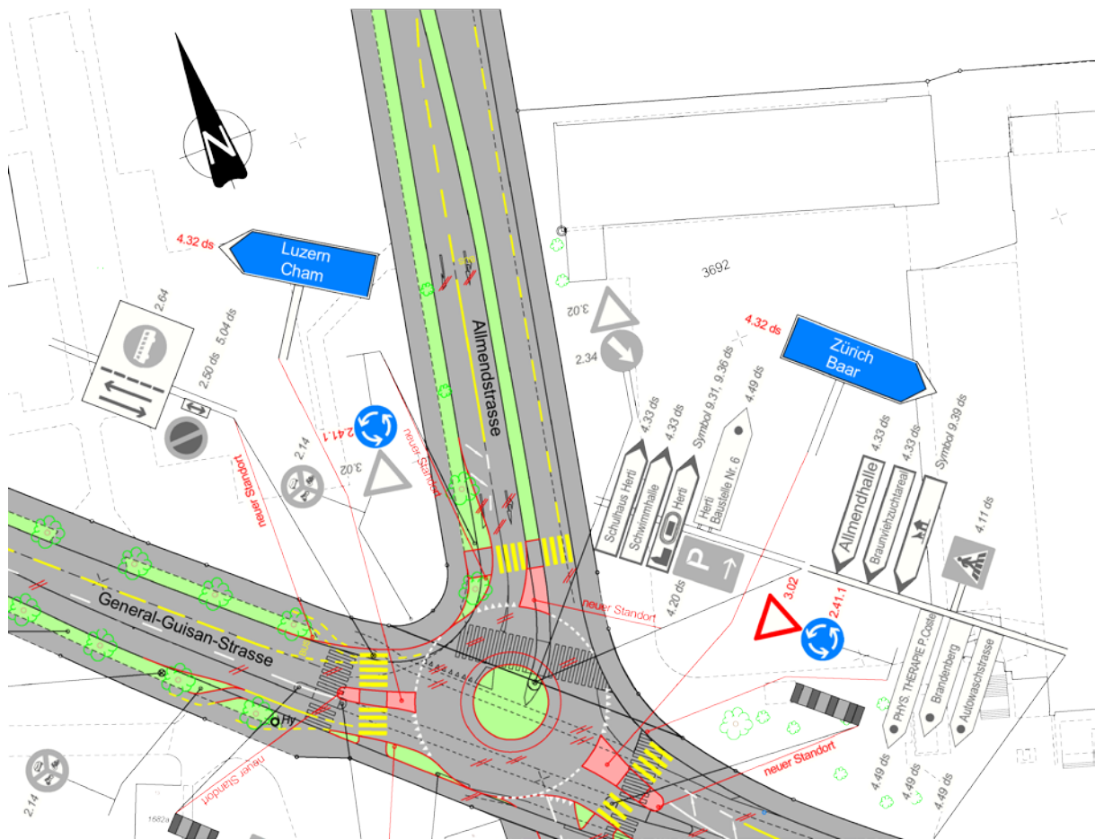
Situationsplan
