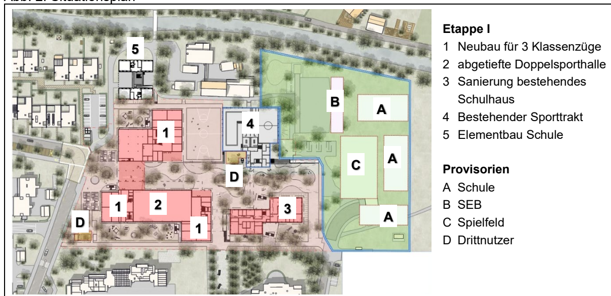
Abb. 2: Situationsplan
